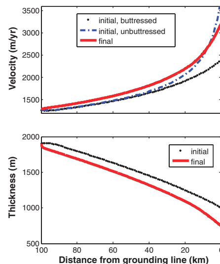
Fig. 4. Modeled response of an idealized version of Pine Island Glacier, West Antarctica, to loss of a small ice shelf (one resisting half of the tendency for ice spreading at the grounding line), following (32). In this model, response is limited to the ice stream itself and cannot propagate into the ice sheet beyond the ice stream. The near-instantaneous increase in velocity following ice-shelf loss is physical but is not simulated in older models lacking longitudinal stresses. The subsequent velocity evolution is largely a result of the thinning and stress reduction in response to that near-instantaneous speedup.
