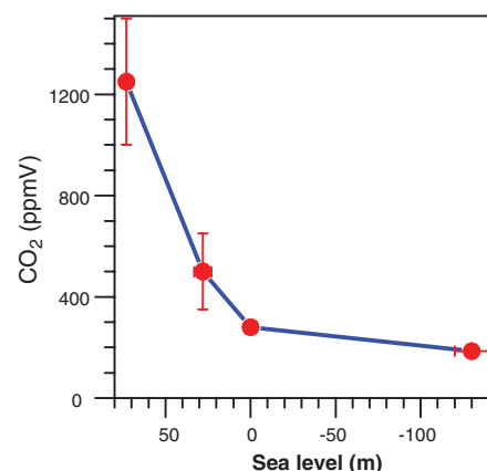
Fig. 1. Relation between estimated atmospheric CO 2 and the ice contribution to eustatic sea level indicated by geological archives and referenced to modern (pre-Industrial Era) conditions [CO 2 = 280 parts per million by volume (ppmV), eustatic sea level = 0 m]. The most recent time when no permanent ice existed on the planet (sea level = +73 m) occurred >35 million years ago when atmospheric CO 2 was 1250 ± 250 ppmV (54). In the early Oligocene (~32 million years ago), atmospheric CO 2 decreased to 500 ± 150 ppmV (54), which was accompanied by the first growth of permanent ice on the Antarctic continent, with an attendant eustatic sea-level lowering 45 ± 5 m (55). The most recent time of low atmospheric CO 2 (185 ppmV) (56) corresponds to the Last Glacial Maximum 21,000 years ago, when eustatic sea level was -130 ± 10 m (8). Error bars show means ± SD.
