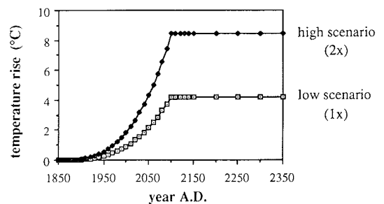
Fig. 6. The temperature scenario's ('high' and 'low') used to force the mass balance and ice dynamics models. The lower curve (1x) is the 'Villach II scenario', the upper curve (2x) corresponds to a temperature rise twice as much.
