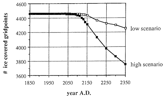
Fig. 9. Evolution of the ice sheet area expressed in number of (#) ice covered gridpoints. 1 gridpoint represents an area of 400 km 2 .
