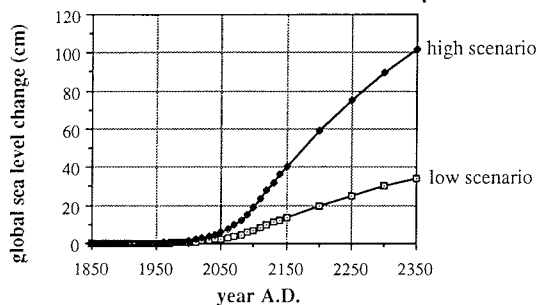
Fig. 7. Response of the ice sheet expressed in global sea level changes. In this experiment, ice dynamics are not considered ('static effect').
