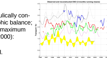
Fig. 5: DSO transport time series 1996–2006. Magenta: Kögu5- \Psi_{\text{Stern}} , Yellow: residual transport, here empirically determined from Iceland Sea NCEP wind stress (1yr, 2 yrs low pass). Black: Reconstructed transport \Psi_{\text{Stern}} + wind stress. Compare with direct observations: ADCP A+B+C, ADCP A only, Angmagssalik array UK1+UK2.
