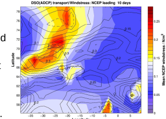
Fig. 6: Correlation of DSO transport 1999-2004 and NCEP wind stress (leading 10 days; black contours and labels). Colours in background: Average NCEP wind stress. Highest amplitude of correlated wind stress in Denmark Strait and Iceland Sea.
