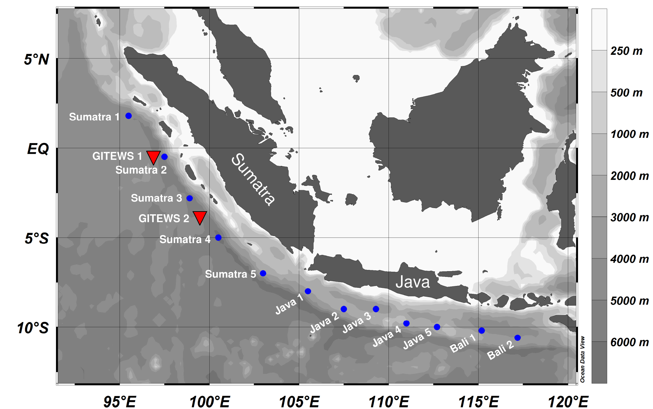
Fig. 7: Proposed GITEWS deployment positions off Indonesia [9]. Triangles mark two surface moorings already deployed in 2005. Sumatra 1-5 and Java 1-5 (dots) are scheduled for deployment in April 2009, five of these with PACT.
