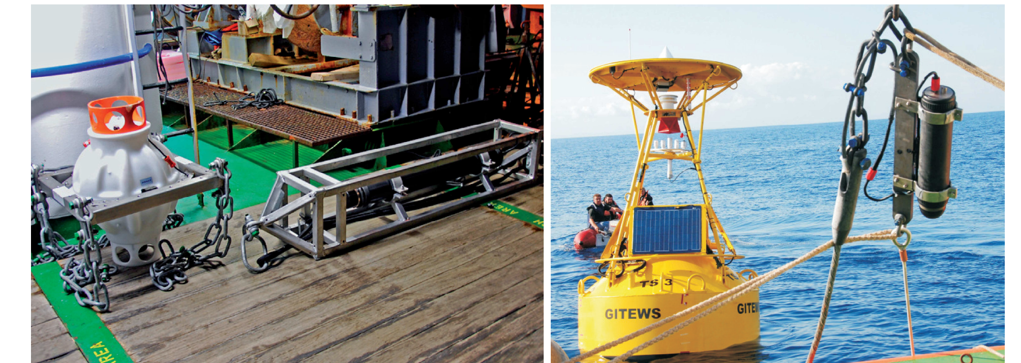
Fig. 6: Left: PACT and HAM.NODE modem prepared for a short-term at-sea test, attached to the ship's hydrographic wire. Right: Test deployment of GITEWS GPS buoy with HAM.NODE modem.
