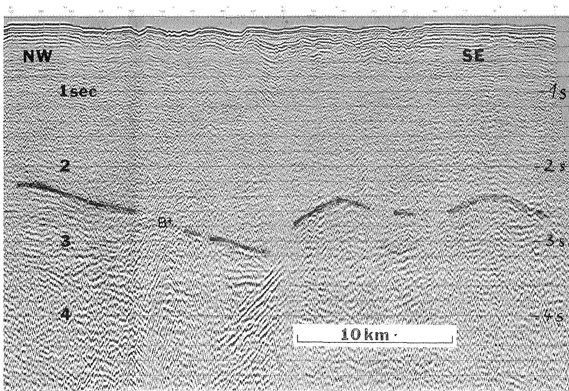
Fig. 10: Reflection seismic record (part of BGR-line 30) of the inner Spitsbergen shelf off Prins Karls Forland. Letter B' as in Fig. 7.
