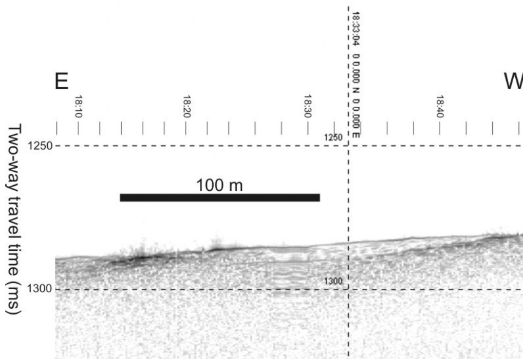
Figure 6: TOPAS profile along the Amundsen Sea continental slope collected with beam steered towards slope while trawling. The profile shows a lenticular body about 185 m wide by up to 5 m thick that is interpreted as having been deposited by a small debris flow. Such small flows may be the basic building blocks of many polar continental slopes, but are unlikely to be identifiable on profiles collected at normal survey speed with a vertically-directed beam.
