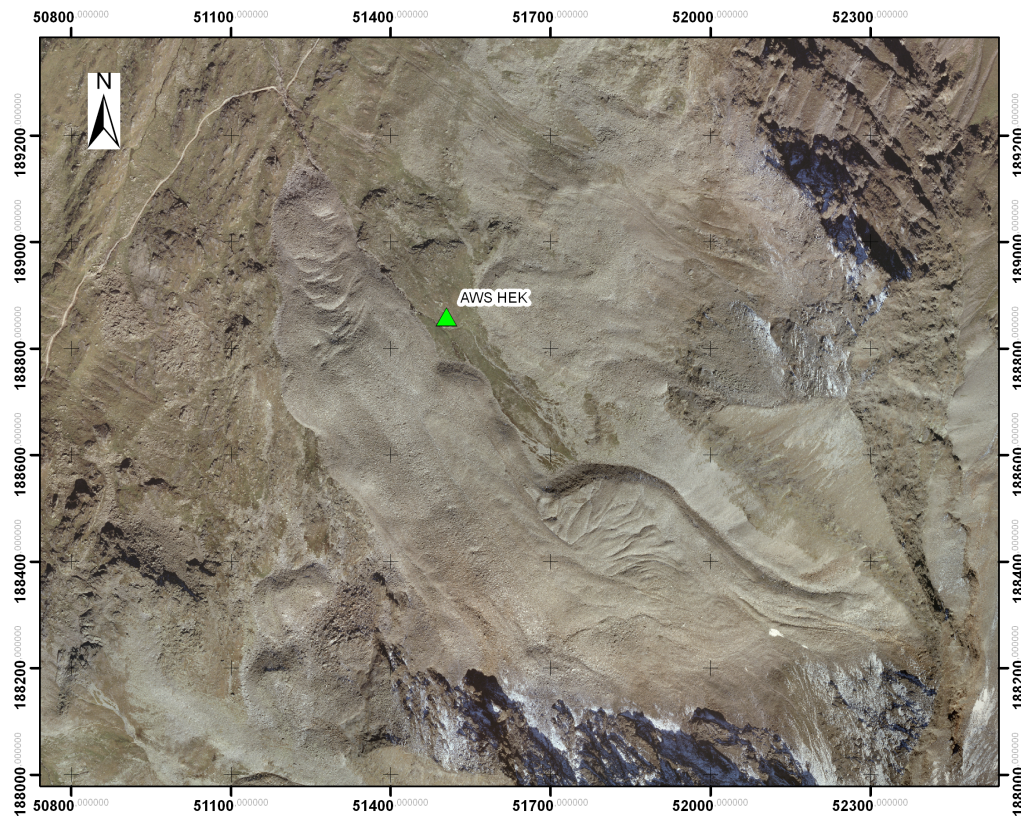
Figure 2.1: Overview: Hochebenkar rock glacier and the location of the AWS. Coordinate system: GK M28
