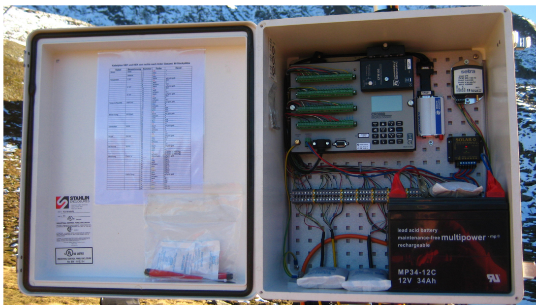
Figure 2.5: Enclosure of the AWS Hochebenkar.
