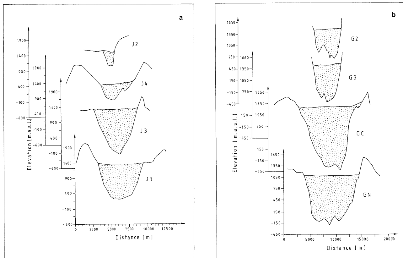
Fig. 4. Cross-profiles (from south to north) of Jenningsbreen (a) and Gjelbreen (b).
