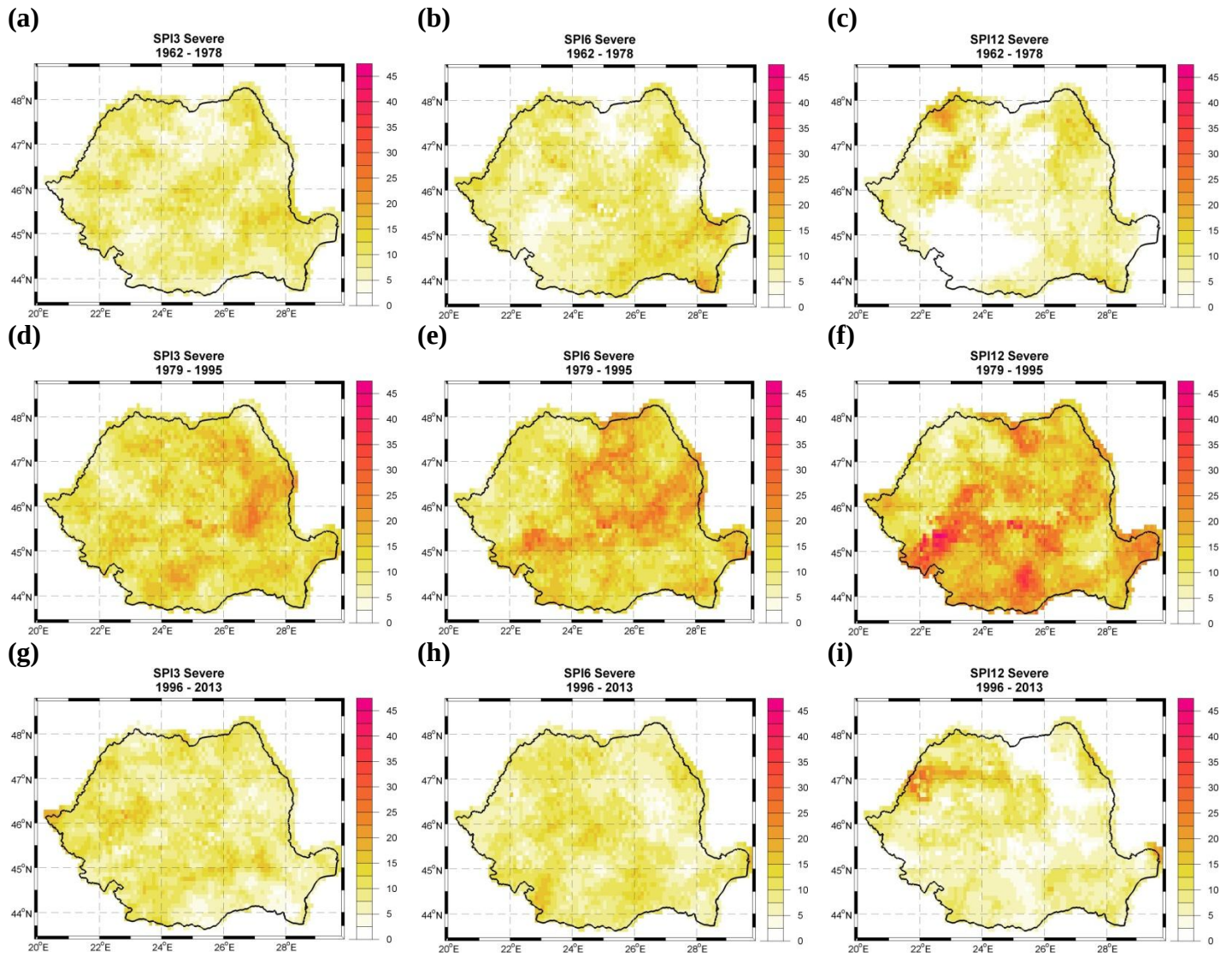
Figure 4. Total severe drought ( -2 < \text{SPI} \leq -1.5 ) duration maps over different periods of time [1962 – 1978 (first row), 1979 – 1995 (second row) and 1996 – 2013 (third row)] and for three different SPI times scales [SPI3 (first column), SPI6 (second column) and SPI12 (third column)].
