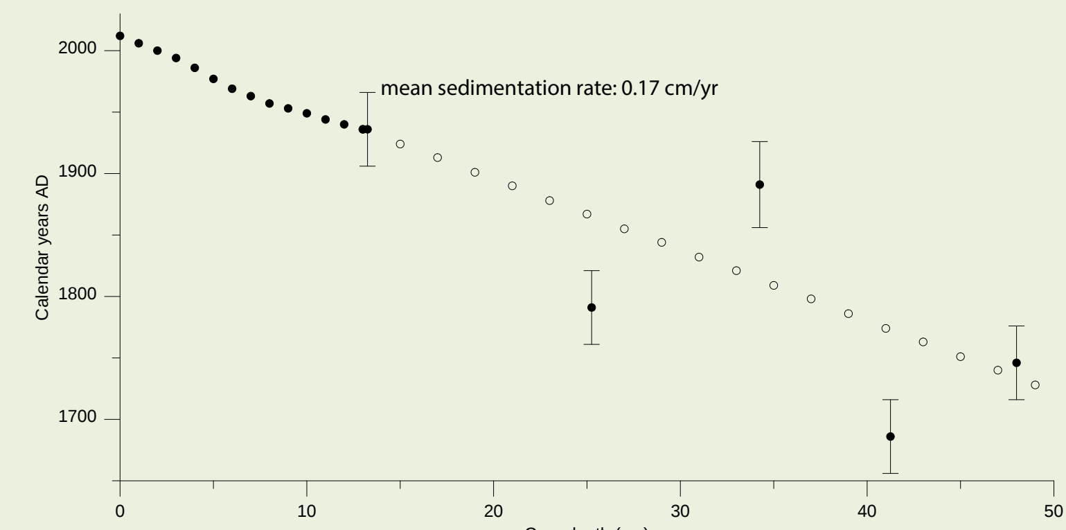
Figure 4. Age depth model based on ^{210}\text{Pb}/^{137}\text{Cs} dating. The filled dots represent ^{210}\text{Pb}/^{137}\text{Cs} dates, the open dots are extrapolated from the mean of dated samples. Dots with error bars represent AMS ^{14}\text{C} dates which are within a similar range but show a much higher uncertainty and were not used in the age model.
