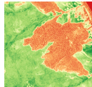
Planet NDVI
