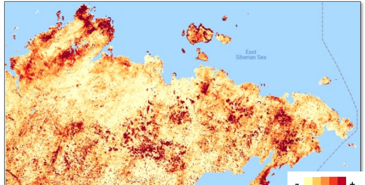
Disturbance by Magnitude for 1999-2020 by LandTrendr
