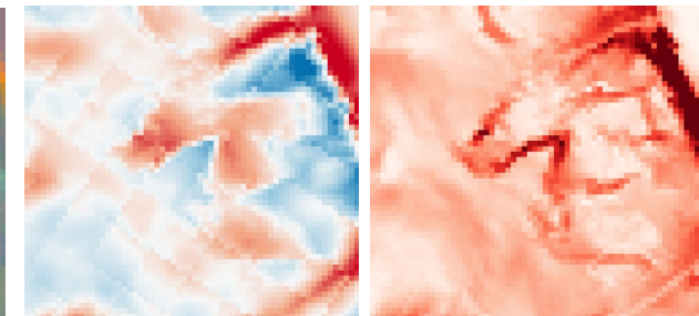
Slump characteristics in Planet data and ArcticDEM
