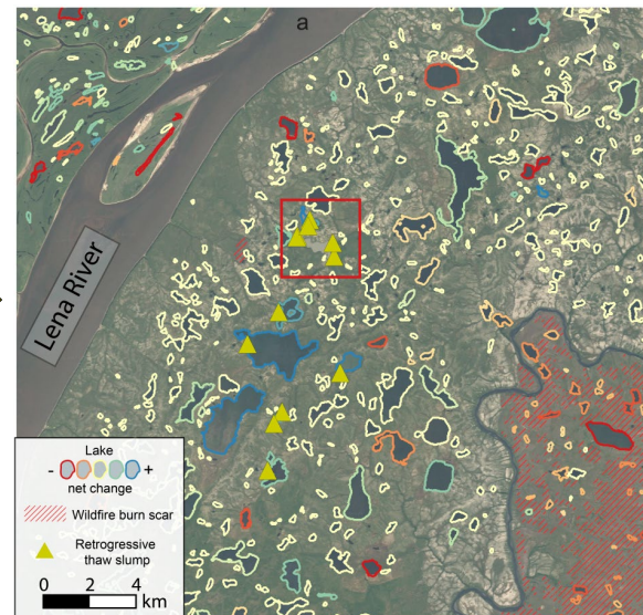
Local example of lake changes, retrogressive thaw slumps and wildfire burn scars along the Lena River, NE Siberia.
