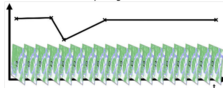
Temporal segmentation by LandTrendr, modified after Kennedy et al. 2010.
