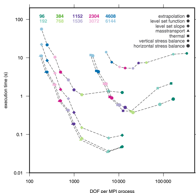
Figure 10. Execution time for matrix assembly for various modules. Symbols are representing the modules, while the colour is denoting the number of MPI processes.
