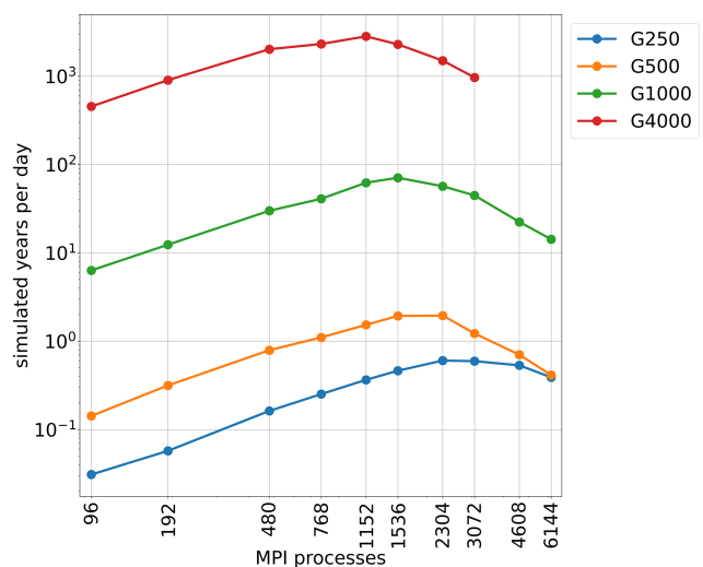
Figure 8. SYPD for various grid resolutions estimated from a run-time of 20 time steps.
