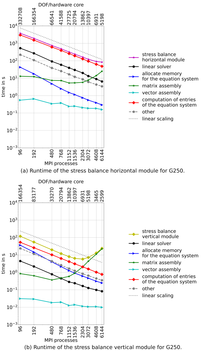
Figure 4. Runtime of the stress balance computation of ISSM Greenland model G250.
