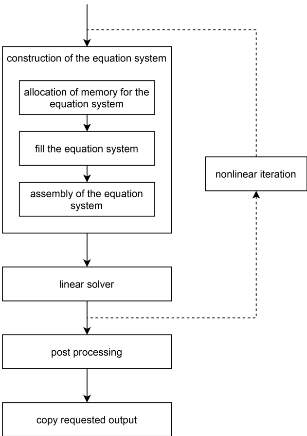
Figure 2. Sketch of a solution sequence of ISSM.
