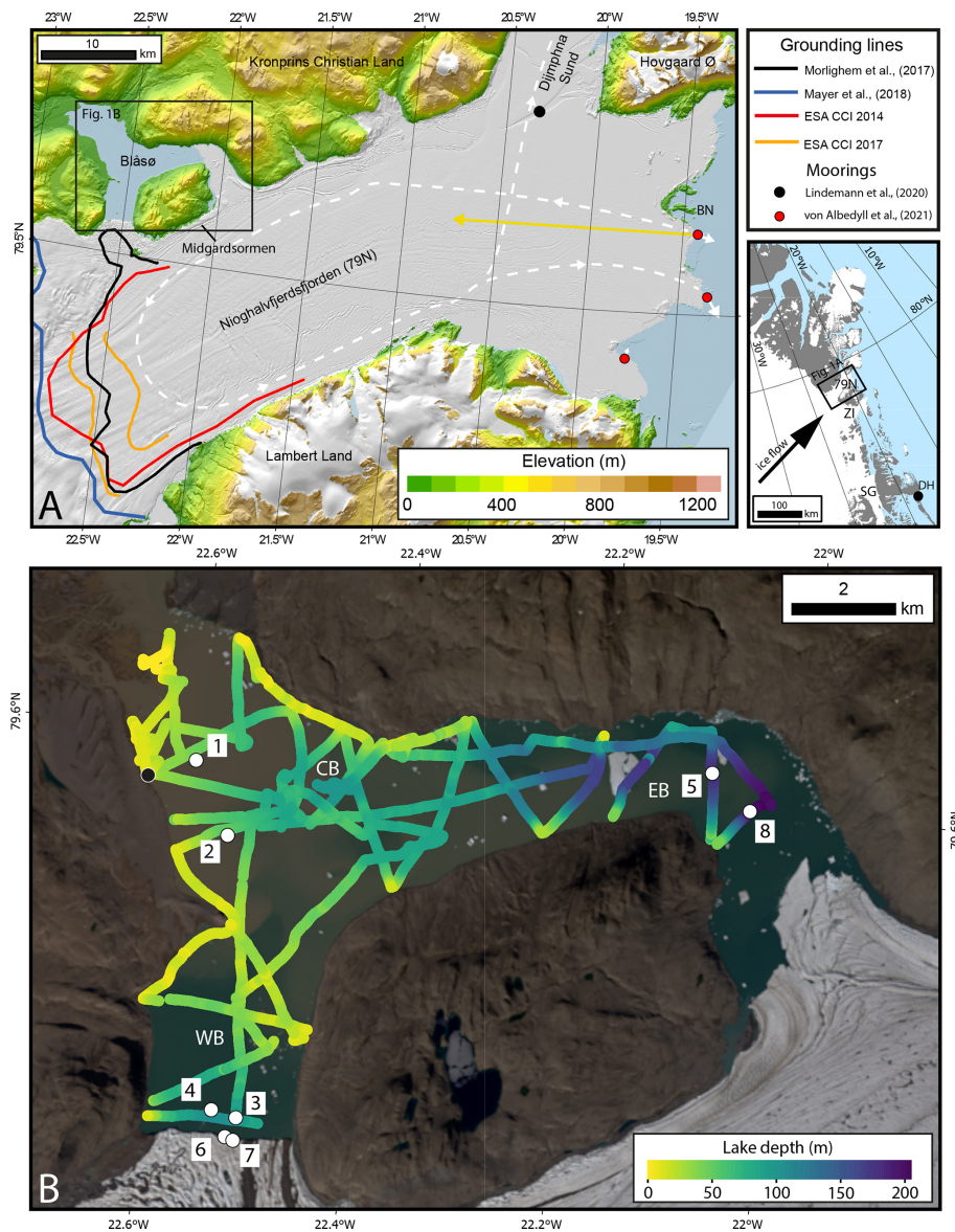
Figure 1. Location map of Blåse. (a) Nioghalvfjærdsfjorden floating ice shelf and the location of Blåse on its northern side, and the 79° N Glacier grounding line (Mayer et al., 2018; Morlighem et al., 2017; ESA CCI v.1.3) in the context of regional topography from the ArcticDEM (Porter et al., 2018). Black dot marks the location of rift mooring of Lindeman et al. (2020). BN represents Bloch Nunatak. Red dots show where moorings have measured flow direction in (yellow arrow) and out (white arrows) of the cavity. Arrow lengths are scaled by current speed (von Albedyll et al., 2021). Dashed lines show a potential cavity circulation (von Albedyll et al., 2021). Inset shows location of Fig. 1a, ZI represents Zachariae Isstrøm, SG represents Storstrømmen Glacier, and DH represents Danmarkshavn. (b) Blåse bathymetry and CTD locations. Colour ramp along transect lines shows surveyed water depths using CHIRP and demonstrates the presence of a western basin (WB), central basin (CB), and eastern basin (EB) in relation to the western and eastern calving fronts. Locations of numbered CTD sites are shown as white dots, and the tide gauge is shown as a black dot. Satellite image is from Landsat 8, from 2 August 2020. Note that during July and August 2017 the eastern end of the lake S and E of the site of CTD8 was occupied by floating lake ice, the edge of which was close to the bathymetric survey line passing through CTD8, and thus the depth of water at the eastern calving margin is not known.
