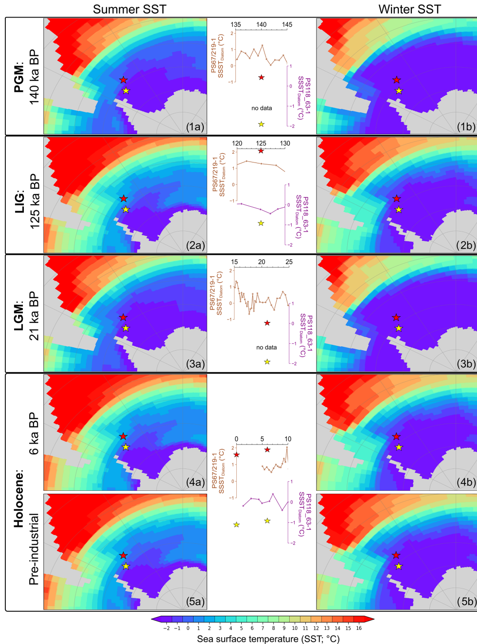
Figure 6. Model-simulated mean (a) summer (DJF) and (b) winter (JJA) sea surface temperature (SST) for the various time slices: (1) PGM, 140 ka; (2) LIG, 125 ka; (3) LGM, 21 ka; (4) mid-Holocene, 6 ka; and (5) pre-industrial. Marine sediment cores, PS118_63-1 (yellow) and PS67/219-1 (red), are indicated by the colored stars. The diatom-based summer sea surface temperature (SSST Diatom ) at both core locations is presented in the middle panel. The corresponding model-simulated SST at each core site (yellow and red stars) for each time slice is displayed alongside the proxy data for comparison.
