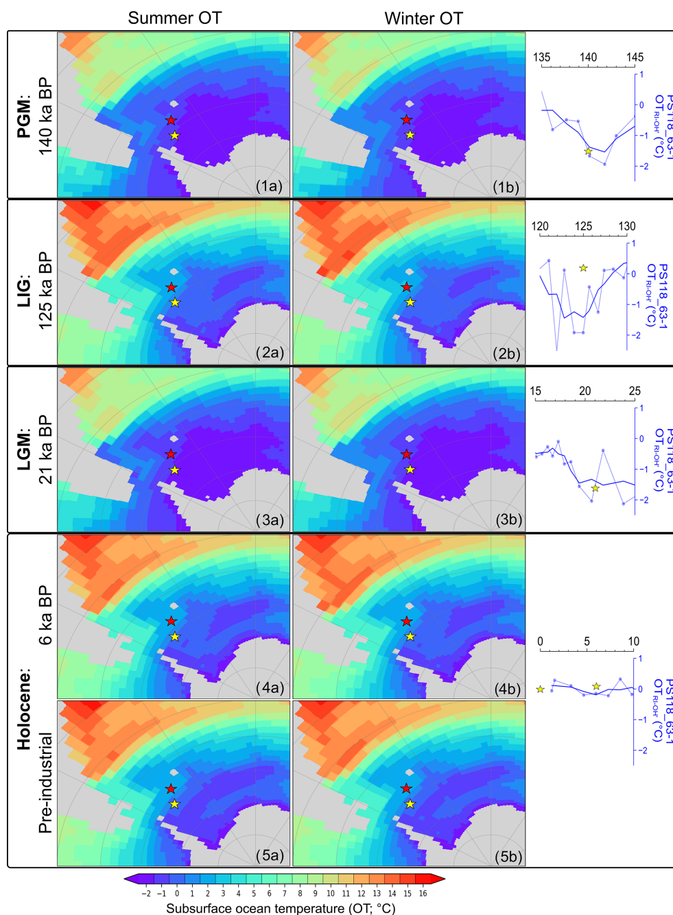
Figure 7. Model-simulated mean (a) summer (DJF) and (b) winter (JJA) subsurface ocean temperature (OT; 220 m water depth) for the various time slices: (1) PGM, 140 ka; (2) LIG, 125 ka; (3) LGM, 21 ka; (4) mid-Holocene, 6 ka; and (5) pre-industrial. Marine sediment cores are presented as colored stars: PS118_63-1 (yellow) and PS67/219-1 (brown). Biomarker-based ocean temperature with three-point smoothing ( OT_{RI-OH'} ) for core PS118_63-1 is presented in the right panel. For comparison, the model-simulated OT for core PS118_63-1 (yellow star) for each time slice is included alongside the proxy-derived OT.
