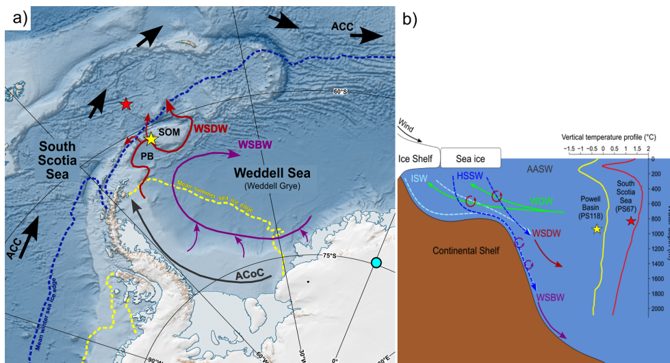
Figure 1. (a) Map of the study area showing the locations of marine sediment cores PS118_63-1 (yellow star) and PS67/219-1 (red star) and the EDML ice core (light-blue circle) discussed in this paper. The mean winter and summer sea ice extents (1981–2010; Fetterer et al., 2017) are illustrated by blue and yellow dotted lines, respectively. The map was adapted from the Norwegian Polar Institute's QAntarctica package using QGIS 3.28 (Matsuoka et al., 2018). (b) Diagram of the Weddell Gyre water masses with vertical spring/summer temperature profiles collected near our core sites in the Powell Basin ( -61.125^{\circ}\text{S} , -47.675^{\circ}\text{W} ) and in the southern Scotia Sea ( -57.125^{\circ}\text{S} , -42.375^{\circ}\text{W} ; World Ocean Atlas 18; Locarnini et al., 2018). Pathways of ocean currents (ACC: Antarctic Circumpolar Current – black; ACoC: Antarctic Coastal Current – gray) and water masses (ISW: ice shelf water – light blue; HSSW: high-salinity shelf water – blue; WDW: Warm Deep Water – green; WSDW: Weddell Sea Deep Water – red; WSBW: Weddell Sea Bottom Water – dark magenta) are represented by the colored arrows. AASW: Antarctic Surface Water; PB: Powell Basin; SOM: South Orkney Microcontinent.
