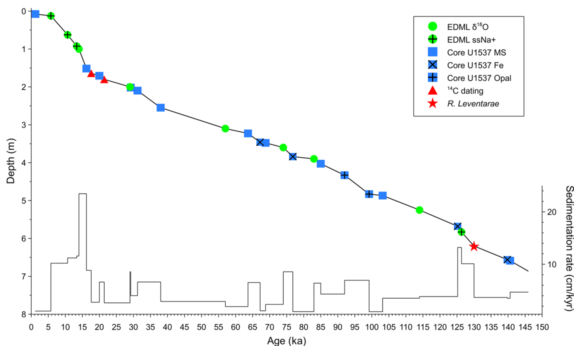
Figure 2. Tie points used for the age–depth model of PS118_63-1 and sedimentation rates. EDML ice core data are indicated by green circles, marine core U1537 data are marked by navy blue squares, and available AMS ^{14}\text{C} dates and the biostratigraphic marker ( R. leventerae ) from core PS118_63-1 are depicted by red triangles ( ^{14}\text{C} dates) and a red star ( R. leventerae ).
