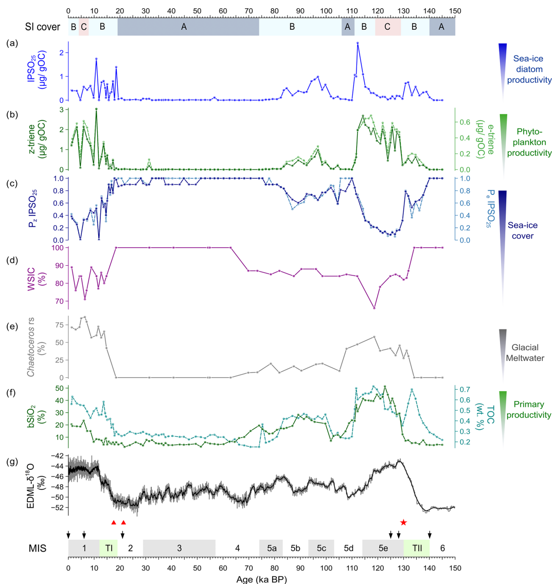
Figure 3. Multiproxy analyses of sea ice conditions in the Powell Basin, reconstructed from marine sediment core PS118_63-1. Sea ice (SI) cover scenarios: A – permanent sea ice cover (dark blue), B – dynamic sea ice cover (light blue), and C – minimal sea ice cover (light red). From top to bottom: (a) HBI-based sea ice biomarker (IPSO 25 ), (b) HBI-based phytoplankton biomarkers ( z -/ e -trienes), (c) phytoplankton-IPSO 25 index (PIPISO 25 ), (d) diatom-based winter sea ice concentration (WSIC), (e) glacial meltwater indicator ( Chaetoceros resting spores), and (f) biogenic opal (bSiO 2 ) and total organic carbon (TOC). Atmospheric temperature is implied by (g) the \delta^{18}\text{O} record from the EDML ice core. AMS 14 C dates are marked with red triangles, and the biostratigraphic marker ( R. leventerae ) is indicated by the red star. The black arrows delineate the time slices for the model simulations in this study. MIS stages are depicted in alternating gray (odd) and white (even) shades, while the terminations TI and TII are shown in green.
