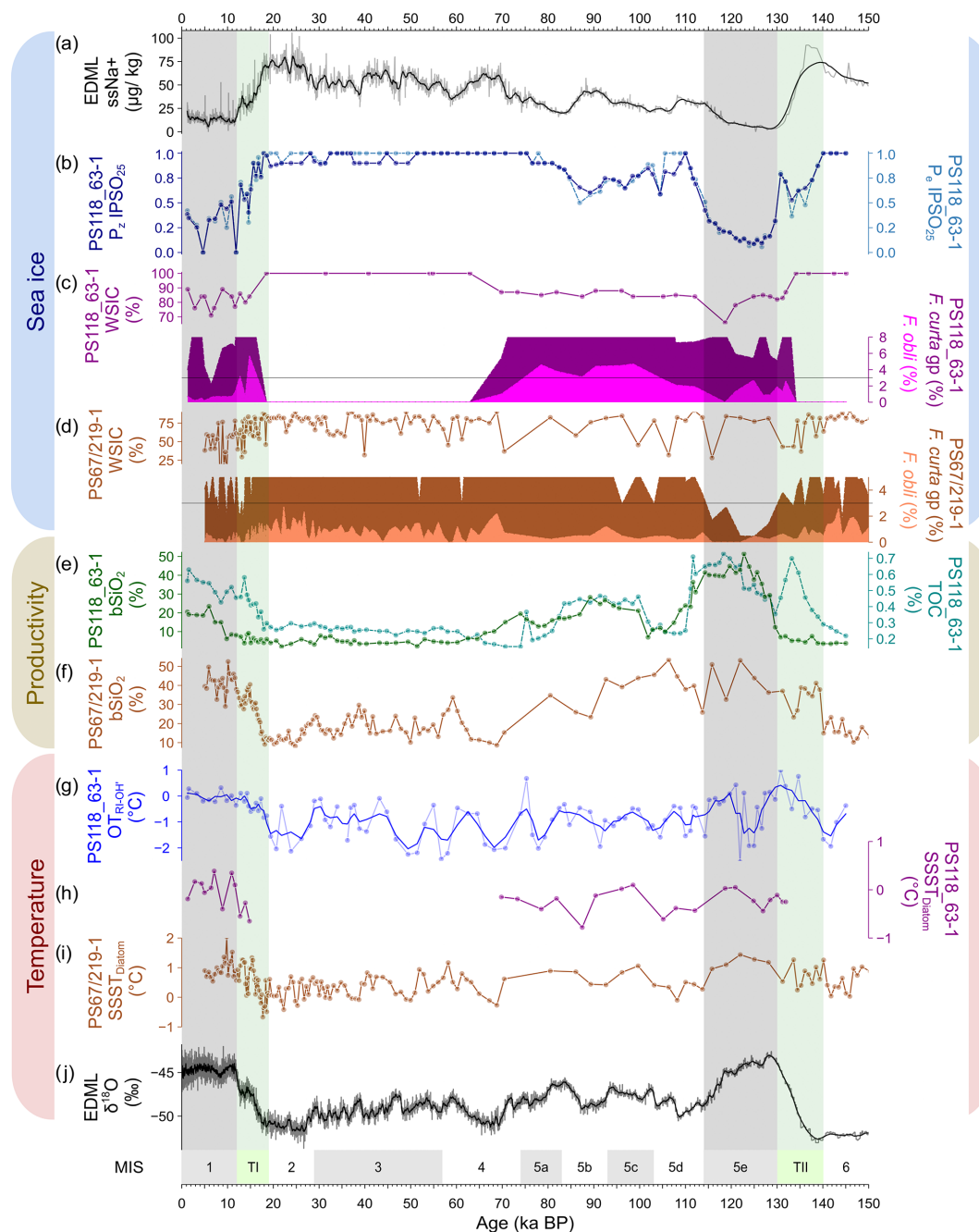
Figure 4. Regional sea ice, productivity, and temperature variability in the South Atlantic sector of the Southern Ocean as inferred from the EDML ice core, the Powell Basin (PS118_63-1), and the southern Scotia Sea (PS67/219-1). For sea ice: (a) sea ice estimation (ssNa+; black) from the EDML ice core; (b) HBI-based sea ice indicator ( P_2\text{IPSO}_{25} – dark blue; P_e\text{IPSO}_{25} – dotted light blue); (c) diatom-based winter sea ice concentration (WSIC – dark magenta), with the F. curta group ( F. curta gp – dark magenta) and F. obliquecostata ( F. obli – light magenta) from PS118_63-1; and (d) diatom-based WSIC (brown), with the F. curta group ( F. curta gp – brown) and F. obliquecostata ( F. obli – light brown) from PS67/219-1. For productivity: (e) biogenic opal (bSiO 2 – dark green) and total organic carbon (TOC – dotted light green) from PS118_63-1 and (f) bSiO 2 (brown) from PS67/219-1. For temperature: (g) RI-OH'-derived subsurface ocean temperature with three-point smoothing (OT RI-OH' – navy blue) and (h) summer sea surface temperature (SSST Diatom – dark magenta) from PS118_63-1, (i) SSST Diatom (brown) from PS67/219-1, and (j) the EDML water stable isotope record ( \delta^{18}\text{O} – black). The 3 % threshold for the relative abundance of diatom species is indicated by a horizontal black line. MIS stages are depicted in alternating gray (odd) and white (even) shades, while the terminations TI and TII are shown in green. For the full F. curta gp abundance data, refer to the relevant datasets in PANGAEA (refer to Data availability).
