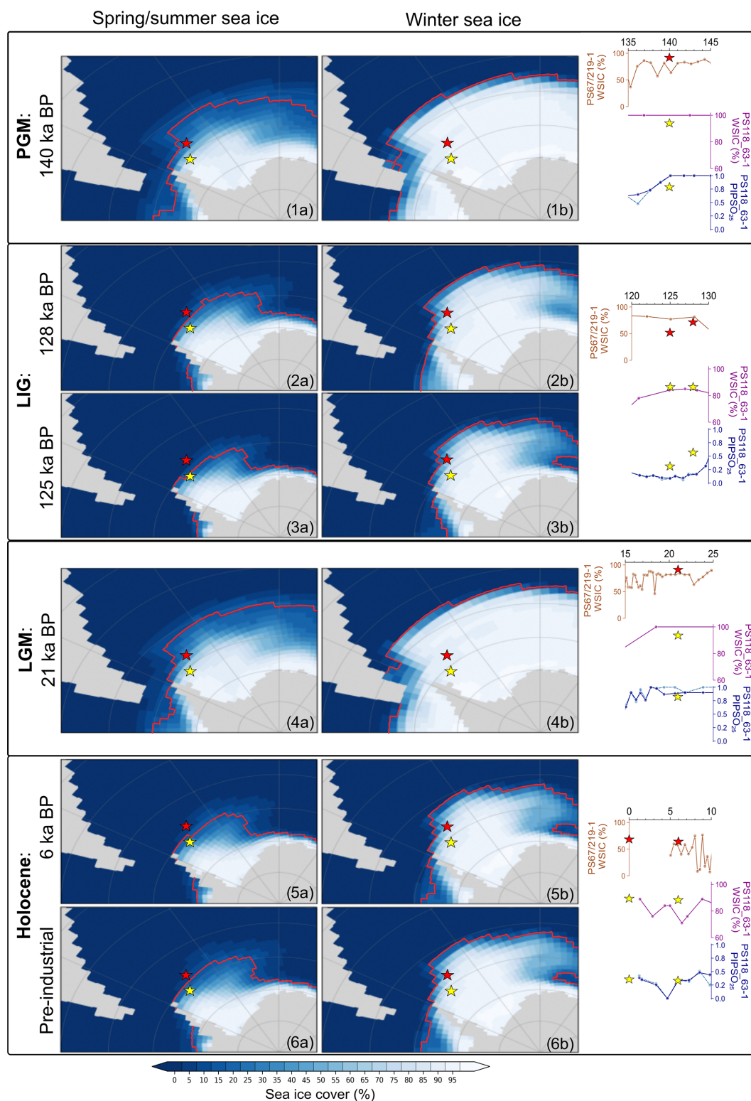
Figure 5. Model-simulated mean (a) spring/summer (NDJFMA) and (b) winter (ASO) sea ice cover for the various time slices: (1) PGM, 140 ka; (2) LIG, 128 ka; (3) LIG, 125 ka; (4) LGM, 21 ka; (5) mid-Holocene, 6 ka; and (6) pre-industrial. The red line depicts the sea ice extent and is defined as the isoline of 15 % sea ice coverage. Locations of marine sediment cores are indicated by stars: PS118_63-1 (yellow) and PS67/219-1 (red). The proxy-derived winter sea ice concentration (WSIC) and spring/summer sea ice (PIPSO 25 ) at each core location are shown in the right-hand column. Additionally, model-simulated sea ice values at each core site (yellow and red stars) for each time slice are plotted alongside the proxy data for comparison.
