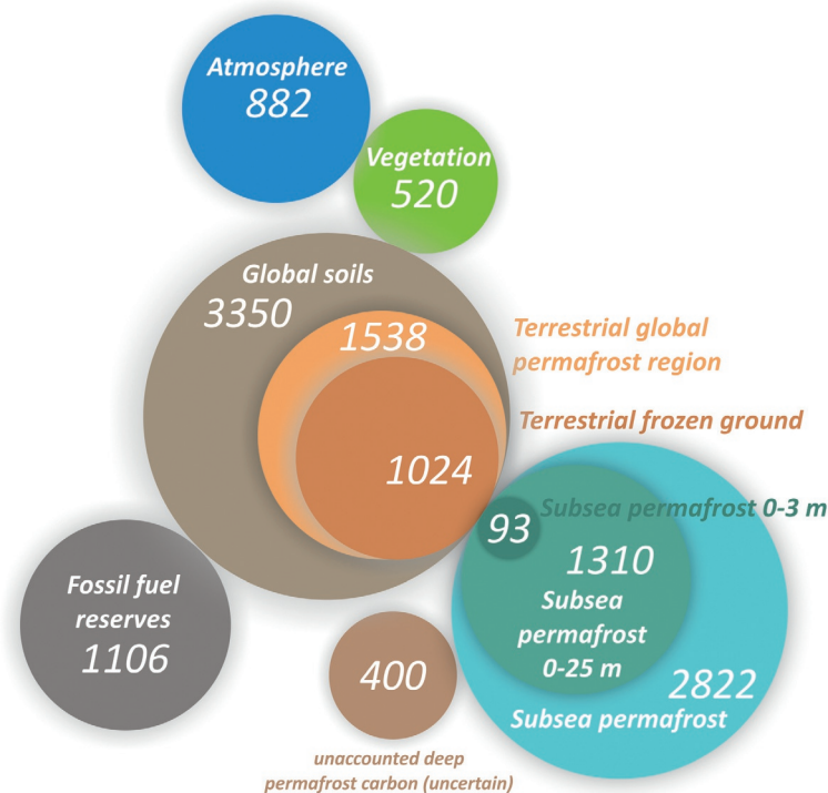
Fig. 3 Terrestrial carbon stocks and atmospheric carbon in relation to the carbon stored in the permafrost region. The size of the circles is proportional to the size of the carbon stock. The C stocks are given in Gt. The global soil estimate (3350 Gt) is based on soils to 3 m depth (2800 Gt) as well as other pools in deep permafrost (500 Gt) and tropical peatlands (50 Gt; Jackson et al., 2017). Based on data from different International Panel on Climate Change (IPCC) reports (e.g., IPCC (2019), Miesner et al., (2023), and Hugelius et al. (2014, 2020). Adapted and updated from Strauss J, Schirrmeister L, Grosse G, Fortier D, Hugelius G, Knoblach C, Romanovsky V, Schädel C, et al. (2017) Deep Yedoma permafrost: A synthesis of depositional characteristics and carbon vulnerability. Earth-Science Reviews 172: 75–86. https://doi.org/10.1016/j.earscirev.2017.07.007 .
