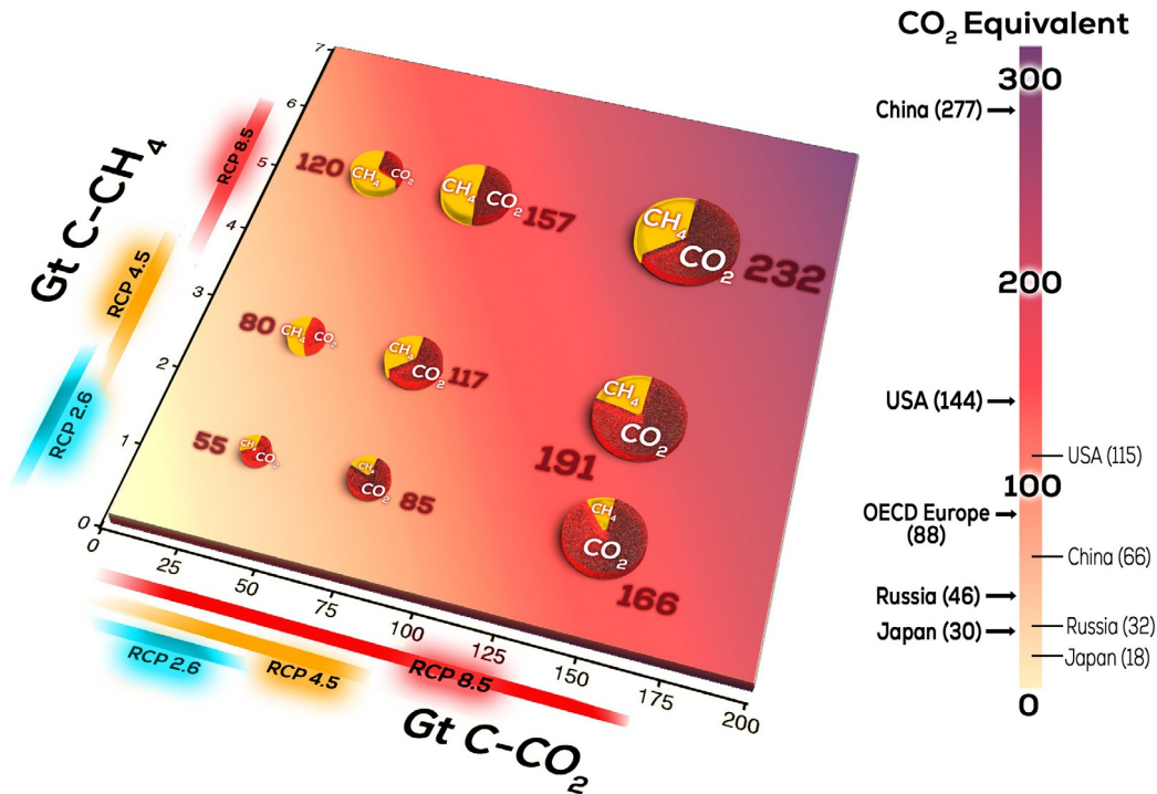
Fig. 5 Visualization of nine scenarios illustrating the cumulative projected emissions of greenhouse gases over the period 2000–2099. These scenarios are based on three levels of net CO 2 emissions (low, medium, high) and three levels of net CH 4 emissions (low, medium, high) into the atmosphere. The x- and y-axes represent the cumulative mass of carbon (in gigatons) contained in either CO 2 or CH 4 , in addition to the preindustrial background carbon exchange. The color scale represents the total greenhouse gas equivalents, measured in gigatons of carbon as carbon dioxide equivalent (Gt C CO 2 -e) units, taking into account the weighting of CH 4 relative to CO 2 . We also provide comparisons with extrapolated (to the year 2099) 2019 country-level carbon emissions (in Gt C CO 2 -e) on the left side and historical (1850–2021) country-level fossil fuel carbon emissions (in Gt C CO 2 -e) extrapolated to 2099 on the right side for several representative nations. The size of each pie chart corresponds to the total CO 2 -e for each specific scenario, and the cumulative Gt C of CO 2 -e labeled under each pie chart shows the relative contributions of CO 2 and CH 4 to the total CO 2 -e. It is important to note that these nine scenarios, for which emissions were quantified, do not cover the upper limits of the CO 2 and CH 4 emissions axes. There remains a possibility of upper-end scenarios, either higher or lower, that fall outside the range depicted in these nine scenarios after a decade of projections. Modified from Schuur EAG, Abbott BW, Commane R, Ernakovich J, Euskirchen E, Hugelius G, Grosse G, Jones M, et al. (2022) Permafrost and climate change: Carbon cycle feedbacks from the warming Arctic. Annual Review of Environment and Resources 47: 343–371. https://doi.org/10.1146/annurev-environ-012220-011847 , drawn by Victor Leshyk.
