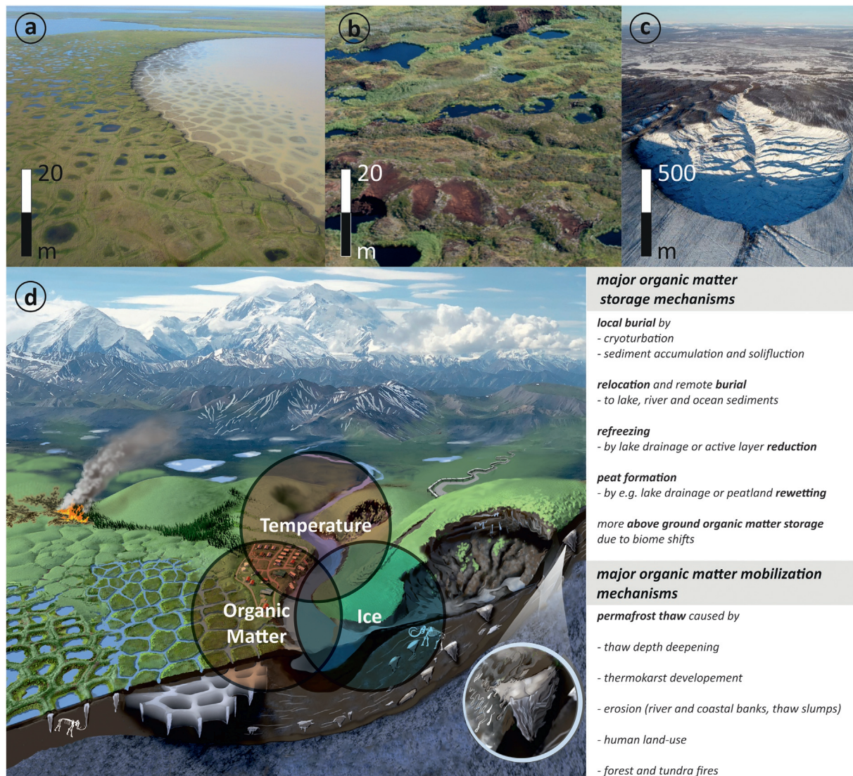
Fig. 2 Permafrost landscape features with a focus on lowland permafrost of the Northern Hemisphere. (A) Thermokarst degradation by lake expansion in northern Alaska. (B) Palsa peatland complex in Tavvavuoma, Sweden. (C) Batagay thaw slump in the boreal zone of Yakutia, Russia. (D) Cartoon of major processes and landscape features with three components (illustrated as overlapping circles) of frozen ground (temperature, ice, and organic matter) that comprise key ecosystem services to people. Temperature (and time) comprise the classical definition of permafrost. The amount of ice determines the structural integrity of frozen ground in the face of permafrost thaw. The amount of organic matter determines the impact on atmospheric composition and climate as the greenhouse gases are released from thawing permafrost (from Schuur et al., 2022, drawn by Victor Leshyk). Images (A) Josefina Lenz, 2018; (B) Matthias Siewert, 2012; and (C) Alexander Kizyakov, 2019. Figure adapted from Strauss J, Abbott B, Hugelius G, Schuur EAG, Treat C, Fuchs M, Schädel C, Ulrich M, et al. (2021a) Permafrost. In: FAO and ITPS (eds.) Recarbonizing Global Soils—A Technical Manual of Recommended Management Practices , pp. 127–147. Rome, Italy: Food and Agriculture Organization of the United Nations.
