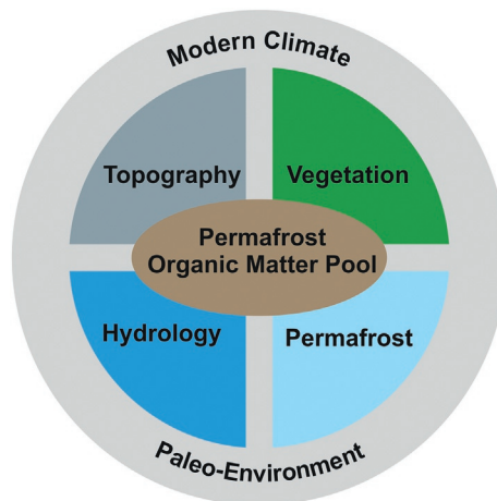
Fig. 1 Major influencing factors of the permafrost organic matter pool. All of these factors not only influence the permafrost organic matter pool, but also interact with each other.
