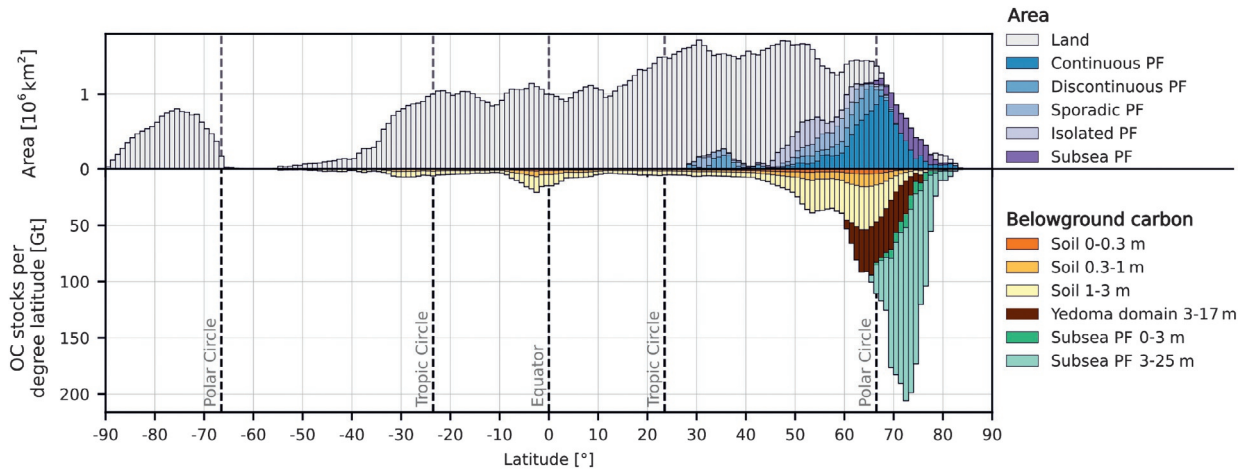
Fig. 4 Latitudinal distribution of belowground organic carbon (OC) in relation to land mass and permafrost coverage. Created with updated data sources (Poggio et al., 2021), different depth classes and including the yedoma regions deep carbon pool (Strauss et al., 2017; Strauss et al., 2021b), as well as the subsea carbon pool (Miesner et al., 2023). The grey and bluish bars on the upper part of the diagram show the area of the land mass per latitude as well as the occurrence of the different types of permafrost (PF) regions. Permafrost from the Southern Hemisphere is not shown in the upper panel.
