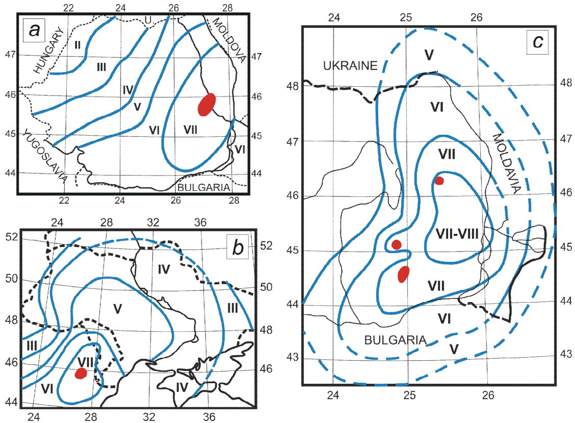
Figure D6. Published isoline maps of the 1990 (main) Vrancea earthquake by: (a) Radu and Utale (1990, 1991); (b) Drumea et al. (2006); (c) Enescu and Enescu (2005, Fig. 4), where PGA is transformed to instrumental intensity, I , with the relation: \log \text{PGA} = 0.2712 \cdot I + 0.1814 . Red zones are the areas of I=VIII .
